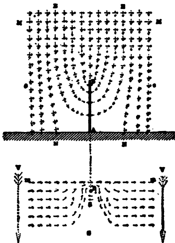
FIG. 24.—Diagrammatic Sections in Elevation and Plan of Electromagnetic Wave Striking a Vertical Conductor while Advancing Towards Observer.
